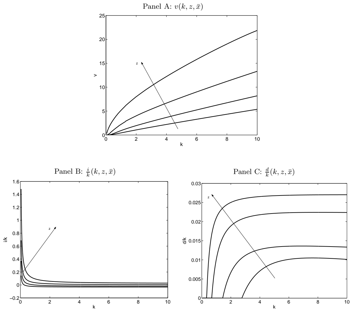
Figure 1 : The Value and Optional Policy Functions
