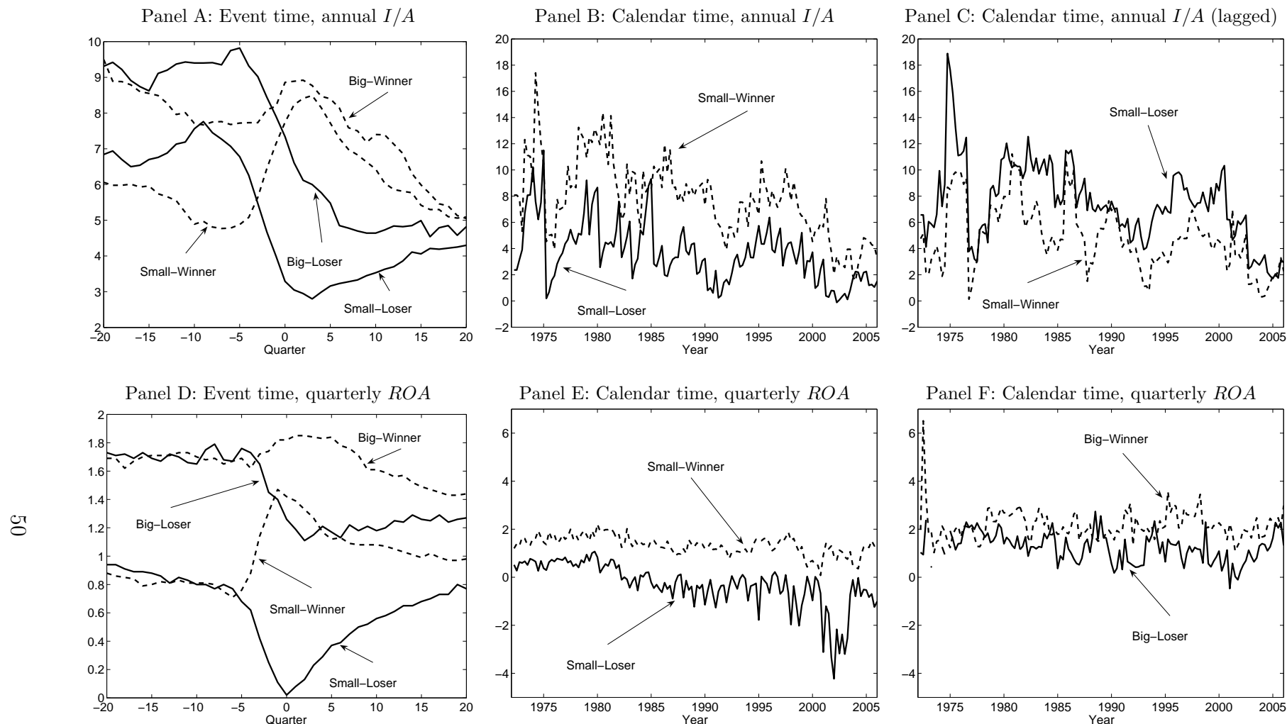
Figure 2. Investment-to-assets ( I/A , contemporaneous and lagged) and ROA for the 25 size and momentum portfolios, 1972:Q1 to 2006:Q4 (140 quarters). We measure I/A as the annual change in gross property, plant, and equipment (Compustat annual item 7) plus the annual change in inventories (item 3) divided by lagged book assets (item 6). ROA is quarterly earnings (Compustat quarterly item 8) divided by one-quarter-lagged assets (item 44). The 25 size and momentum portfolios are constructed monthly as the intersections of five quintiles formed on market equity and five quintiles formed on prior two- to seven-month returns (skipping one month). For each portfolio formation month t , from January 1972 to December 2006, we calculate annual I/A s and quarterly ROA s for t + m, m = -60, \dots, 60 . The I/A and ROA for month t + m are averaged across portfolio formation months t . ROA is the most recent ROA relative to formation month t . Panels A and D plot the median I/A s and ROA s across firms in the four extreme portfolios, respectively. In Panel B I/A is the current year-end I/A relative to month t . In Panel C the lagged I/A is the I/A on which an annual sorting on I/A in each June is based. Panels E and F plot the times series of ROA for the four extreme portfolios.
