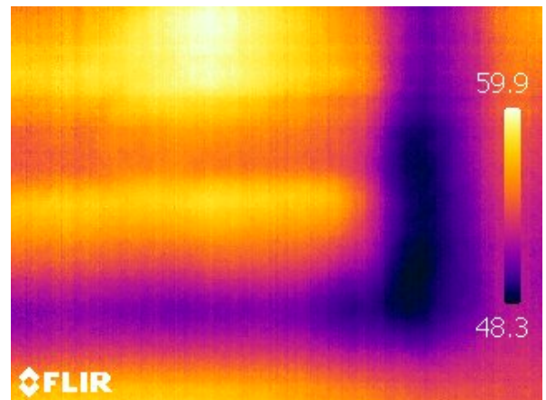
Photo 29 - Thermal Image of Photo 28
